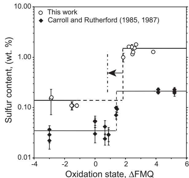
Fig. 3. Comparison of the S concentration as a function of f\text{O}_2 in basaltic melts (at 1300°C and 1 GPa; this work) and in trachyandesites (at 200 MPa and for 927 < T < 1027^\circ\text{C} ; Carroll & Rutherford, 1985, 1987). The data from Carroll & Rutherford (1985, 1987) include only glasses with \text{FeO} < 17 wt % to show only the effect of changes in f\text{O}_2 . The arrow indicates the expected shift in the stability of sulfate phases with decreasing silica activity, based on data from Sisson (2003).
